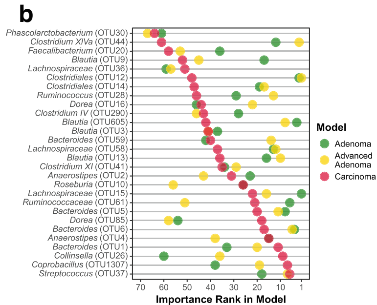
Fig. 3 Top 10% most important OTUs common to those models used to differentiate between patients with normal colons and those with adenoma, advanced adenoma, and carcinoma. a Venn diagram showing the OTU overlap between each model. b For each common OTU the lowest taxonomic identification and importance rank for each model run is shown
